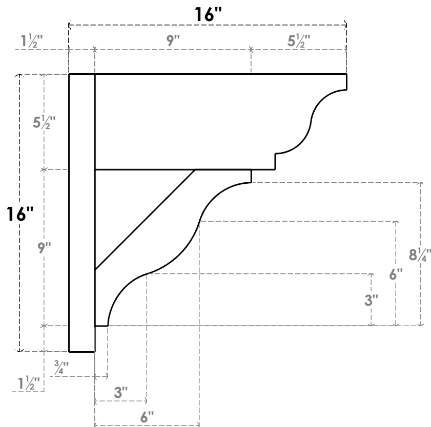
SIDE PROFILE
